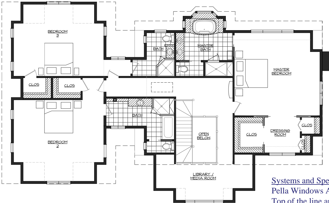
2 nd Floor – 2,042
